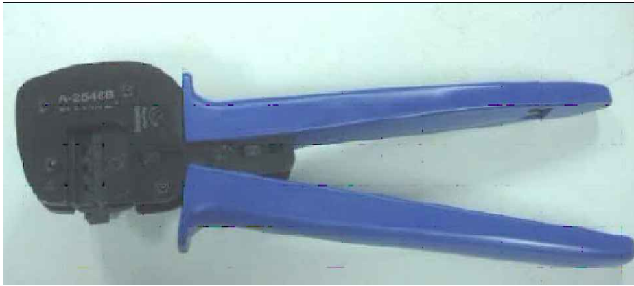
CRIMPING TOOL(CA-AES-CT-15) DIE INSERT AND CRIMPING LOCATOR INCLUDED FOR 10, 12, 14 AWG
