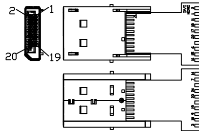
DP CONNECTOR
