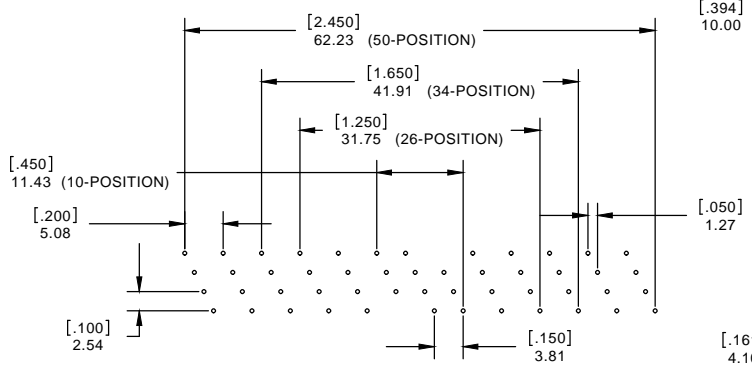
RECOMMENDED PCB LAYOUT FOR 10, 26, 34, 50 POSITION CONNECTOR
