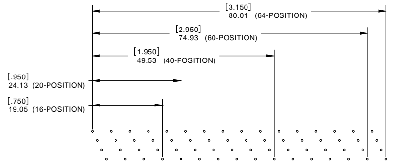
RECOMMENDED PCB LAYOUT FOR 16, 20, 40, 60, 64 POSITION CONNECTOR
