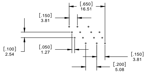
RECOMMENDED PCB LAYOUT FOR 14 POSITION CONNECTOR
